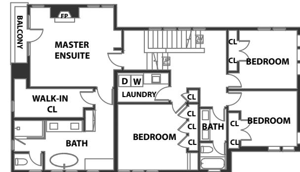
UPPER LEVEL
